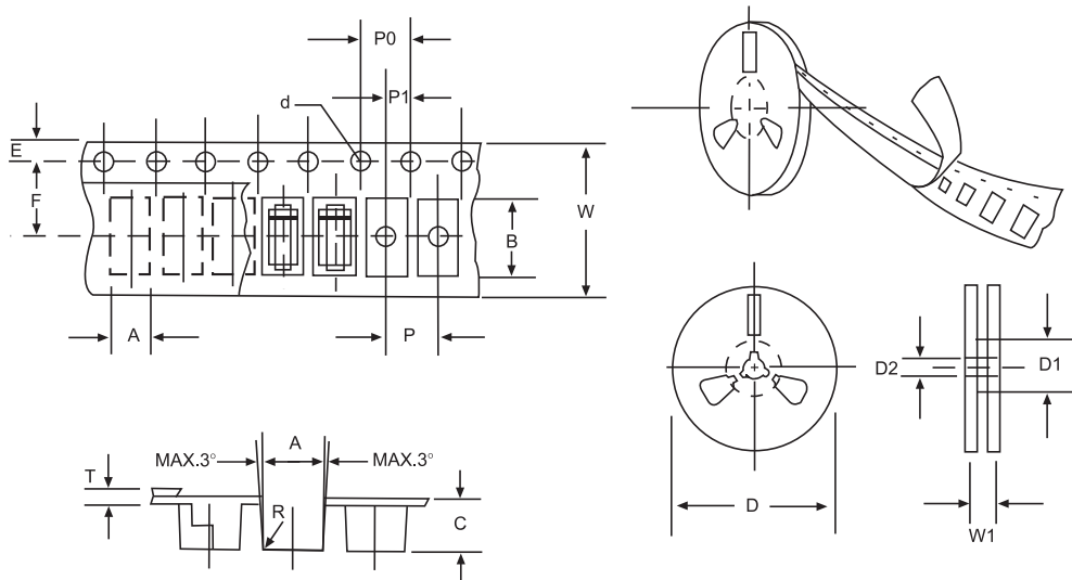
Fig:CONFIGURATION OF FLAT MELF TAPING
